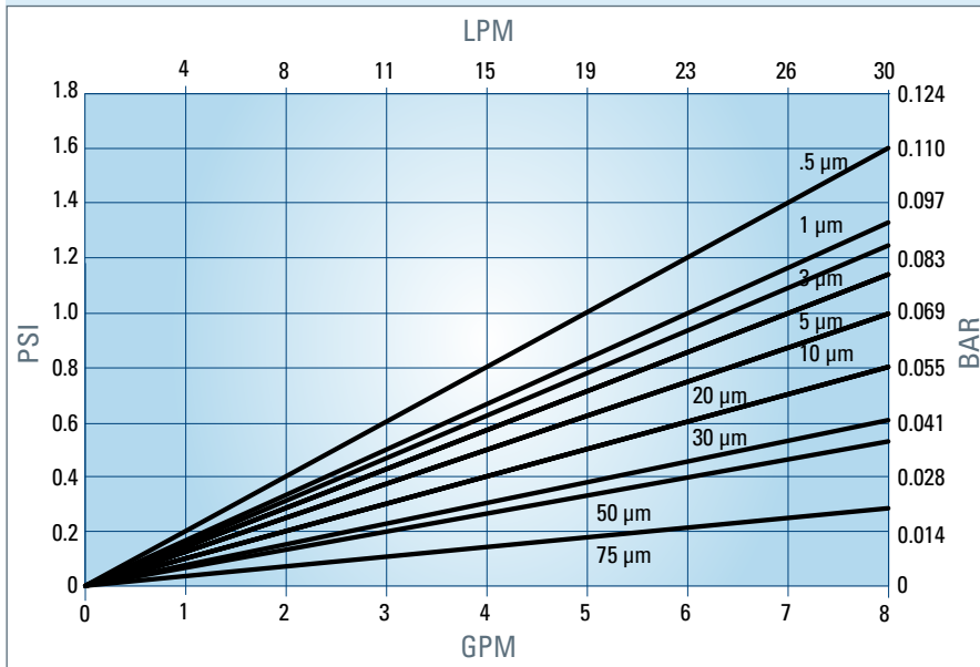
PP-FC 100 DIFFERENTIAL PRESSURE PER 254 MM (TEN INCH) EQUIVALENT (TIE) – WATER
